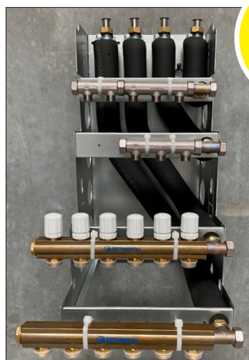
Standard BUNDMODUL: ALBE-BASICPTM-653
